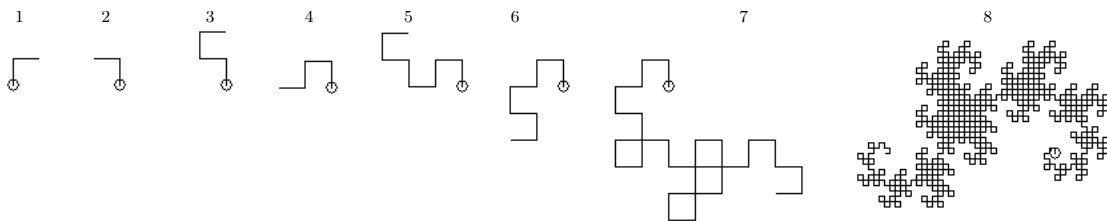
FIGURE II.7 – Courbe du dragon
